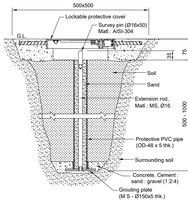
Typical installation schematic
